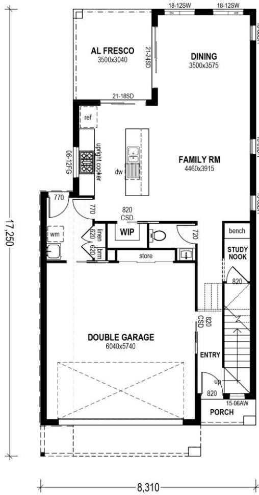
LOWER FLOOR PLAN
